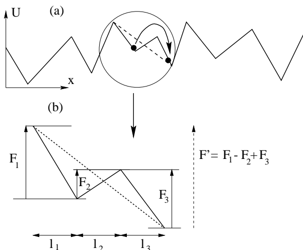
FIG. 1. (a) Energy landscape in the Sinai model (b) decimation method: the bond with the smallest barrier F_{min} = F_2 is eliminated, resulting in three bonds being grouped into a single one.
