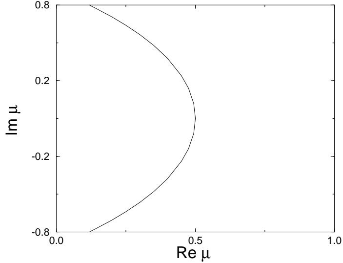
FIG. 5. Stability diagram: the solid line in the complex plane of \mu delimitates the region of instability ( Re(\Phi) < 0 to the right of the line) from the region of stability ( Re(\Phi) > 0 to the left)
