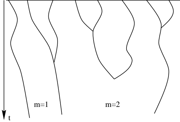
FIG. 11. diffusion and merging of domains. To each domain present at time t (bottom of the figure) is associated the number m of ancestor domains in the initial state (defined at the top slice t = 0 ). Note that some initial domains die without producing any descendant domain at time t .
