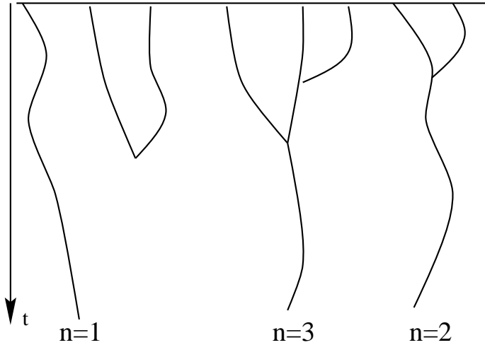
FIG. 15. Number of ancestors of surviving particle.
