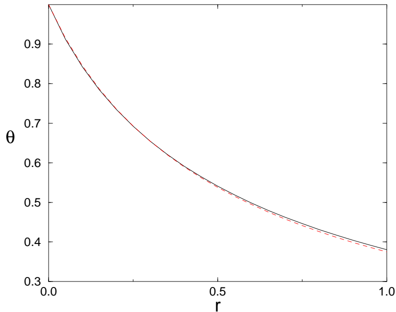
FIG. 9. Plot of \bar{\theta}(r) as a function of r (solid line) and, for comparison, \frac{1}{2}\theta_{pure}(r) (dashed line)
