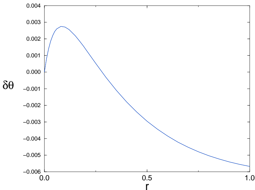
FIG. 10. Plot of \delta\theta(r) = \frac{1}{2}\theta_{pure}(r) - \bar{\theta}(r) : the difference remains very small for all r . It vanishes at r = 0 and r = 0.280701..
