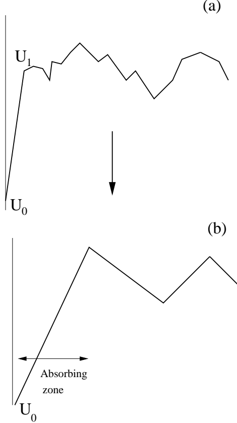
FIG. 7. Illustration of the RG in presence of an absorbing boundary. (a) the boundary at site x = 0 can be represented by setting U_0 = -\infty . (b) renormalized landscape, with the absorbing zone (see text).
