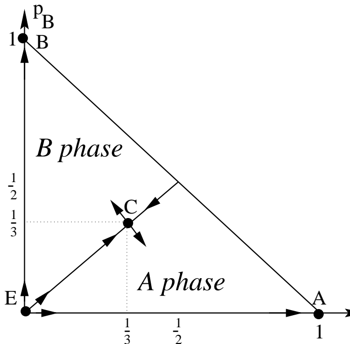
FIG. 6. Dynamical phase diagram of the reaction (59) studied in the text.
