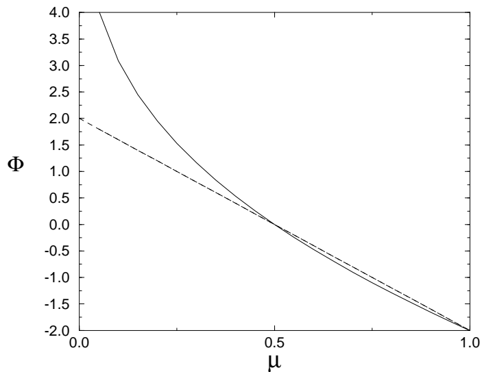
FIG. 3. Plot of the exponent \Phi ( \Phi^- ) as a function of the eigenvalue \mu . It vanishes at \mu = 1/2 and diverges as \mu \rightarrow 0 . The result of the uniform approximation is plotted as a dashed line.
