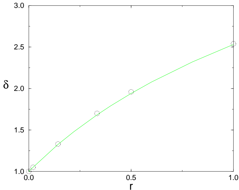
FIG. 12. Plot of the exponent \delta(r) for the process (4) in the Sinai landscape, determined by equation (108) (solid line), and comparison with the numerical results of Krapivsky and Ben Naim (Ref. 46) for the pure case (circles).
