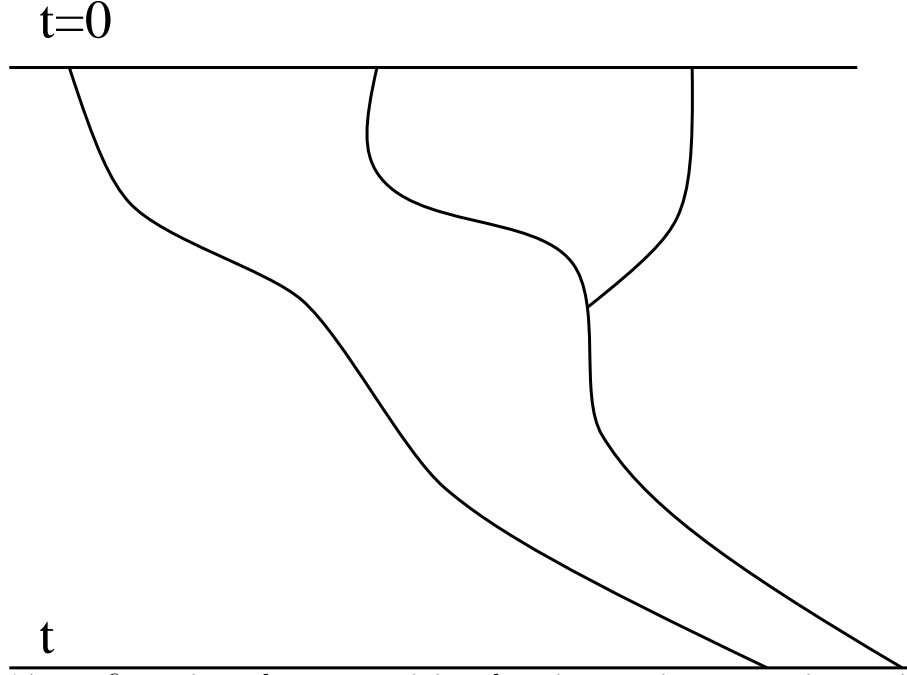
FIG. 14. configuration where a surviving domain contains no persistent site, which accounts for the strict inequality \psi(r) < \bar{\theta}(r) found here for r > 0 .
