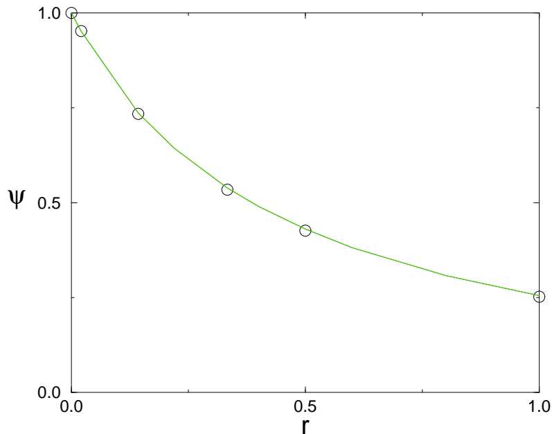
FIG. 13. Plot of the exponent \psi(r) for the process (4) in the Sinai landscape, determined by equation (132) (solid line), and comparison with the numerical results of Krapivsky and Ben Naim (Ref. 46) for the pure case (circles).
