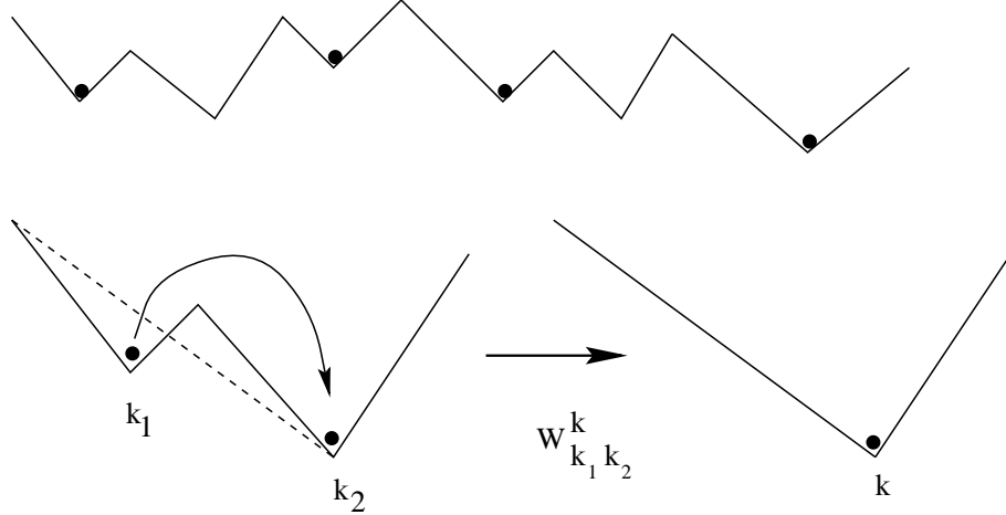
FIG. 2. (a) macroscopic state of the reaction diffusion process: each renormalized valley is either empty ( k = 0 ) or contains a particle of type k > 0 (b) at time scale t such that the barrier F = \Gamma = T \ln t is decimated, the state (particle) k_1 in the decimated valley moves to the neighboring valley and reacts with k_2 to produce k with probability W_{k_1, k_2}^k , as the two valleys are merged into a single renormalized one containing k
