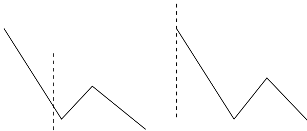
FIG. 8. If the point at x = 0 (indicated by a dotted line) happens to lie in a renormalized valley as shown on the left figure, it will be crossed many times by a single particle, while it may not be crossed at all by the thermal average \langle x(t) \rangle before it jumps over the barrier on the right. This is not the case in the situation shown on the right figure, where typically no crossing of x = 0 occurs for a single particle.
