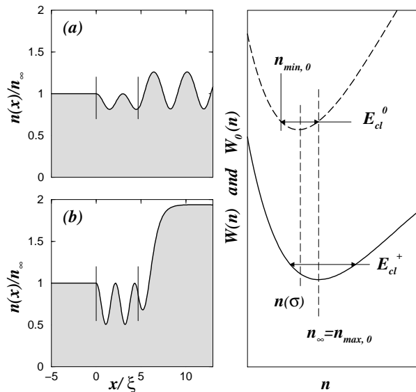
Figure 9: A C-solution in an attractive square well. Left and right parts as in Fig. 3. Both density plots on the left part concern a low density beam, with v_\infty/c_\infty = 1.6 and a square well of width \sigma/\xi = 4.68174 . Plot (a) is the generic case and corresponds to V_0 \xi^2 = 0.1 . For these values of V_0 and v_\infty the condition (32) is fulfilled for any \sigma . Plot (b) corresponds to a well of depth V_0 \xi^2 = 0.5 . The parameters have been chosen in this case such that E_{cl}^+ = W(n_2) and the C-solution is just about to disappear. The right plot illustrates the behavior of the typical solution (corresponding to part (a)) in the diagram (n, W(n)) . The density is constant and equal to n_\infty for x \leq 0 in W(n) . From x = 0 to x = \sigma the “classical particle” evolves in W_0(n) (with an energy E_{cl}^0 ). Finally the up-stream density oscillates in the classical potential W(n) as a cnoidal wave.
