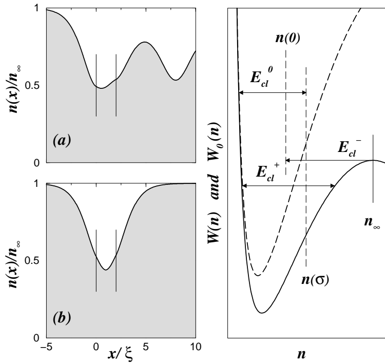
Figure 5: A D_1 solution in an attractive square well. Left and right parts as in Fig. 3. Plot (a) is the generic case (with n(\sigma) > n(0) ) and (b) is the symmetric case where n(\sigma) = n(0) . These plots correspond to \sigma = 2\xi and V_0 \xi^2 = 0.1 in a low density beam at velocity v_\infty/c_\infty = 0.7 . The right plot illustrates the behavior of the typical solution (such as displayed in part (a)) in the diagram (n, W(n)) . The down-stream density evolves from n_\infty to n(0) in the potential W(n) with a classical energy E_{cl}^- = W(n_\infty) . Then in W_0 (with an energy E_{cl}^0 ) from n(0) to the minimum density n_{min,0} and back to a value n(\sigma) (larger than n(0) ). Finally the up-stream density oscillates in the classical potential W(n) as a cnoidal wave.
