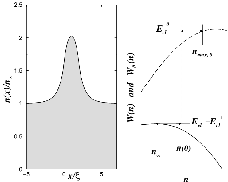
Figure 3: Type-B stationary solution in an attractive square well. The left plot displays the density profile. The two vertical solid lines indicate the location of the square well. This plot corresponds to \sigma = 2\xi and V_0\xi^2 = 0.5 in a low-density beam at velocity v_\infty/c_\infty = 0.7 (the healing length \xi is defined as in (9) and is computed at density n_\infty ). The right plot illustrates the behavior of the solution in the diagram (n, W(n)) . The solid curve represents W(n) and the dashed one W_0(n) . In the rear of the obstacle, the density evolves from n_\infty to n(0) in the potential W(n) with a classical energy E_{cl}^- = E_{cl}^+ , then from n(0) to n_{max,0} and back to n(0) in the potential W_0(n) (with energy E_{cl}^0 ), and finally the up-stream density goes from n(0) to n_\infty in W(n) .
