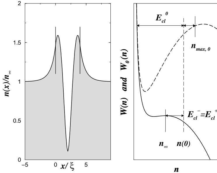
Figure 4: A B_2 solution in an attractive square well. Left and right parts as in Fig. 3. The plot corresponds to \sigma = 4\xi and V_0\xi^2 = 0.5 in a low density beam at velocity v_\infty/c_\infty = 0.7 . The down-stream density evolves from n_\infty to n(0) in the potential W(n) with a classical energy E_{cl}^- = W(n_\infty) , then it makes a complete oscillation in W_0(n) starting from n(0) towards n_{max,0} and ending again at n(\sigma) = n(0) . Finally the up-stream density goes from n(\sigma) to n_\infty in the potential W(n) .
