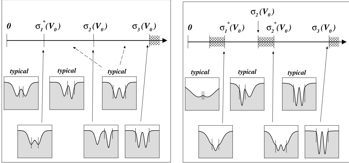
Figure 8: Synoptic diagram of the evolution of the morphology of the D_2 solution for given V_0 , as \sigma increases (see caption of Fig. 7). For \sigma larger than \sigma_3(V_0) the D_2 solution disappears (it becomes a B_3 solution). The left part corresponds to a shallow well and the right part to a deep well. For legibility, the cases denoted as “typical” have been taken to consist ahead of the obstacle (for x \geq \sigma ) of a portion of a soliton (whereas the most generic solutions are cnoidal waves).
