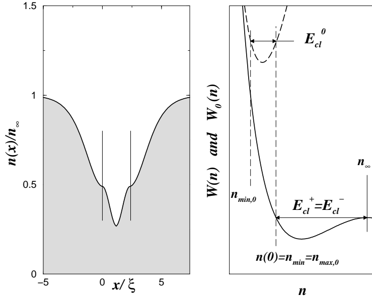
Figure 6: The D_1 solution in a strongly attractive square well of width just above \sigma_1^*(V_0) . Left and right parts as in Fig. 3. The density outside the well is composed of two half solitons. This plot corresponds to V_0 \xi^2 = 0.5 and \sigma \simeq 2.4 \xi in a low density beam at velocity v_\infty/c_\infty = 0.7 . The density evolves from n_\infty (far down-stream) to n(0) = n_{min} in the potential W(n) with classical energy E_{cl}^- = W(n_\infty) . It then evolves in W_0 from n(0) to n_{min,0} and back. Finally the up-stream density oscillates in the classical potential W(n) from n(\sigma) = n_{min} back to n_\infty .
