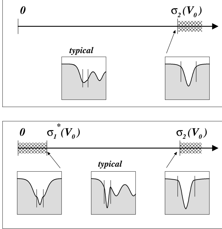
Figure 7: Synoptic diagram of the evolution of the morphology of the D_1 solution for a given V_0 , as \sigma increases. The insets display the density profiles n(x)/n_\infty . Hatched regions indicate values of \sigma for which the solution does not exist. For shallow potentials (for which n_{1,0} > n_{min} , upper part of the plot) the D_1 solution exists for any width \sigma between 0 and \sigma_2(V_0) . For deep potentials ( n_{1,0} < n_{min} , lower part) it exists only if \sigma \in [\sigma_1^*(V_0), \sigma_2(V_0)] . In both cases (shallow or deep potential) at \sigma = \sigma_2(V_0) the D_1 solution disappears and becomes a B_2 solution.
