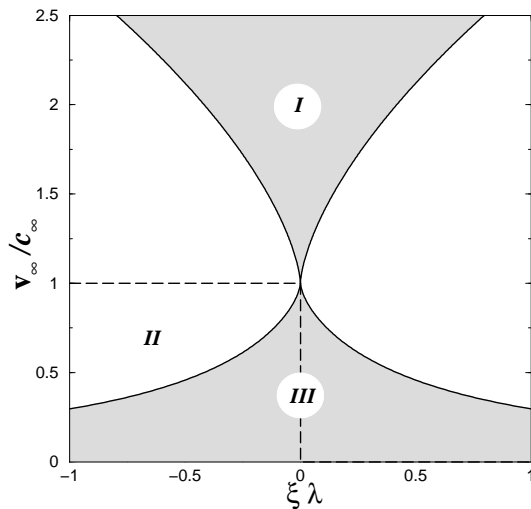
Figure 13: Domains of existence of the different solutions occurring for a dilute beam in a potential V_\parallel(x) = \lambda \delta(x) . Region I occurs only for v_\infty/c_\infty > 1 and corresponds to C-solutions. Region II corresponds to B 1 -solutions and occupies the domain under the dashed line (it occurs only for attractive potentials and for v_\infty/c_\infty < 1 ). Region III corresponds to D-solutions: D 1 -solutions for \lambda > 0 and D 2 solutions when \lambda < 0 .
