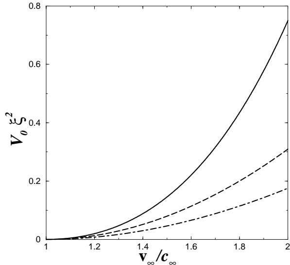
Figure 10: Representation (for low density beams) of the part of the plane (v_\infty, V_0) where the C solution is allowed for any potential width. The allowed region is located below the solid curve. We also display on the same diagram the region where C solutions are allowed for any width of a repulsive potential (see Sec. 6.1). It corresponds to the domain below the dashed curve for low density beams and below the dot-dashed one for high density beams.
