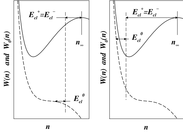
Figure 12: Schematic representation in the (n, W(n)) diagram of the behavior of D_1 -solutions in a strong repulsive square well ( v_\infty/c_\infty < 1 ). The solid curve represents W(n) and the dashed one W_0(n) . For this type of potential there are two possible solutions for a given value of the width \sigma (as discussed in the text). This is illustrated by the figure, namely the “time” the fictitious particle spends in the potential W_0 is the same in the left and right plots. For simplicity, the examples we give here are drawn in the particular case n(0) = n(\sigma) .
