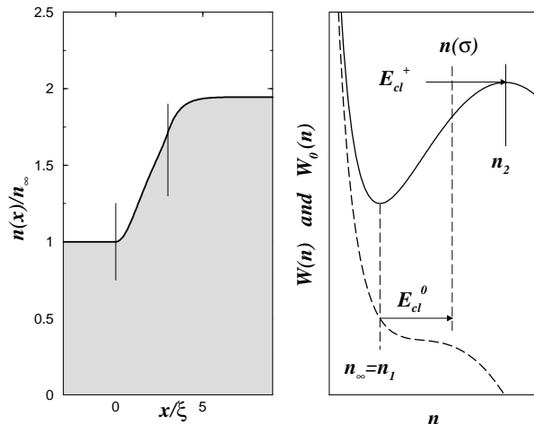
Figure 11: A C-solution in a repulsive square well. The parameters have been chosen in this case such that E_{cl}^+ = W(n_2) and the C-solution is just about to disappear. Left and right parts as in Fig. 3. The left plot concerns a low density beam, with v_\infty/c_\infty \simeq 1.6 and a square well of width \sigma/\xi = 3 and depth V_0 \xi^2 = 0.1 . The right plot illustrates the behavior of this solution in the diagram (n, W(n)) . The down-stream density is constant and equal to n_\infty . From x = 0 to x = \sigma the “classical particle” evolves in W_0(n) (with an energy E_{cl}^0 ), then it evolves back in W(n) , just on the separatrix.
