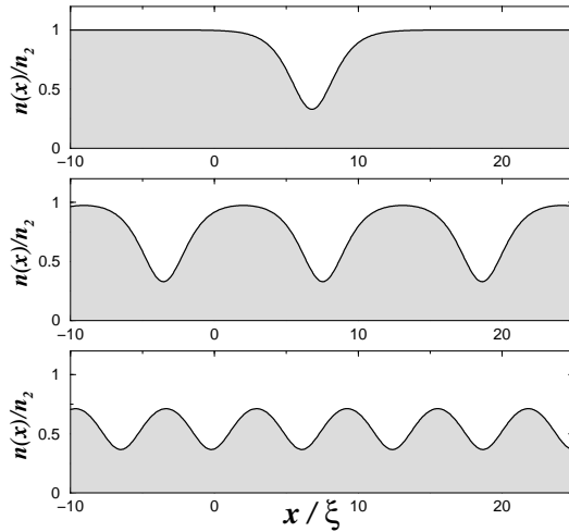
Figure 2: Beam density along a straight guide (high density regime) with v_2/c_2 = 0.7 (lengths are given in units of \xi(n_2) , see Eq. (9)). Top: solitary wave ( E_{cl} = W(n_2) ). Middle: cnoidal waves existing for W(n_1) < E_{cl} < W(n_2) . Bottom: for E_{cl} \gtrsim W(n_1) the cnoidal wave deforms continuously to a sinusoidal small-amplitude wave.
