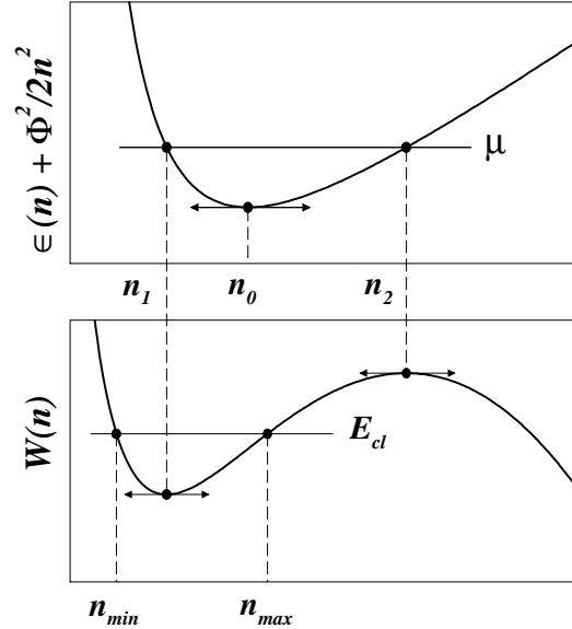
Figure 1: Schematic behavior of the functions \epsilon(n) + \Phi^2/2n^2 (top part) and W(n) (bottom part) as a function of n . n_i ( i = 1 or 2 ) is defined by \epsilon(n_i) + \Phi^2/2n_i^2 = \mu and is a zero of dW/dn ; n_0 is a zero of the second derivative d^2W/dn^2 . For \mu and \Phi given, a beam of uniform density has either a density n_1 (and a velocity higher than the sound velocity c(n_1) ) or a density n_2 (and a velocity lower than c(n_2) ). At a given E_{cl} , n_{min} and n_{max} are the minimum and maximum values of the density oscillations ( W(n_{min}) = W(n_{max}) = E_{cl} ).
