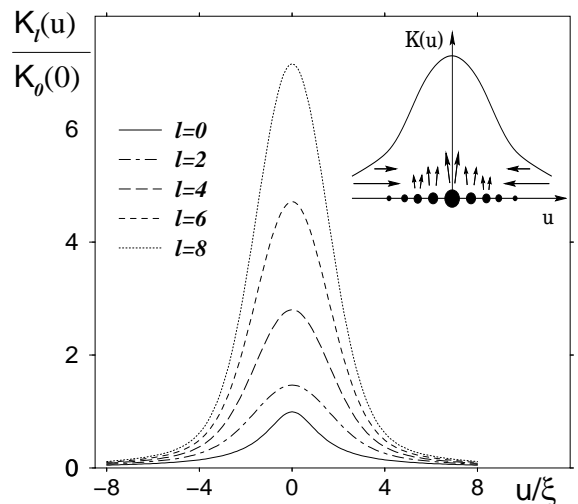
FIG. 1. The high temperature ( \tilde{T} = \xi^2 ) diffusive flow of the correlator K_l(u) evolving under the linearized FRG for n=2 . We choose a bare correlator K_0(u) = \{1 + \ln[1 + (u/\xi)^2]/2\} / [1 + (u/\xi)^2] with non-integrable logarithmic tails as in the vortex problem. After a crossover around l=1 the correlator K_l(0) increases quadratically with l as expected from Eq. (13). The inset schematically illustrates the interplay of the diffusive inflow of “particles” (horizontal arrows) and the “particle” sources originating from the quadratic one-loop terms (solid dots). In the short-range case the first mechanism is absent and K_l grows due to the non-linear terms only, while in the strongly long-range case ( \beta < 2 ), the non-linear terms can be neglected and K_l grows due to the inflow from the tails. The vortex pinning problem is intermediate with a crossover at a scale l_{\text{cr}}(\tilde{T}) < l_c(\tilde{T}) from diffusion driven growth to source driven growth.
