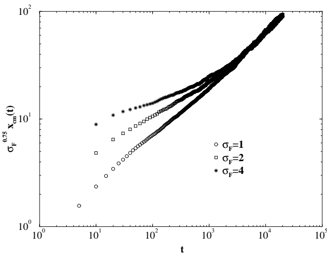
FIG. 3. Behaviour of the average center of mass x_{cm}(t) for different values of \sigma_F . This curves shows that for large \sigma_F , the short time behaviour is Sinai like, crossing over to the mixed behaviour at large times. The value of x_{cm}(t) has been rescaled by \sigma_F^{3/4} to obtain a reasonable data collapse at large times.
