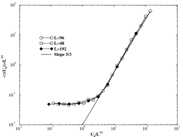
FIG. 4. Average barrier crossing time \langle \tau \rangle , rescaled by L^{3/2} , as a function of the barrier height U_0 rescaled by \sqrt{L} , for different sizes L , and in log-log coordinates. The slope 5/3 is shown for comparison. The power law increase of \langle \tau \rangle as a function of U_0 has to be compared to the usual exponential (activated) dependence.
