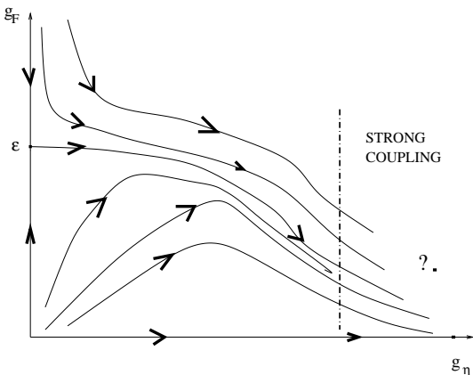
FIG. 1. One loop RG flow in the g_\eta, g_F plane. As soon as g_\eta is non zero, it flows towards the strong coupling region. Our numerical simulations suggest that an attractive ‘mixed’ fixed point appears in this region.
