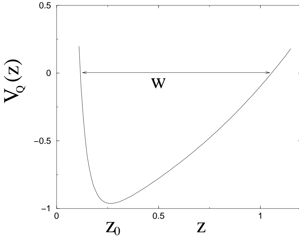
FIG. 2. The shape of the potential V_Q(z) in Eq. (C7) is shown for parameter values: a = 1 , \nu' = 0.5 and p = 0.1 . The potential has a minimum at z = z_0 \sim p and a typical width W \sim p in the limit p \rightarrow 0 .
