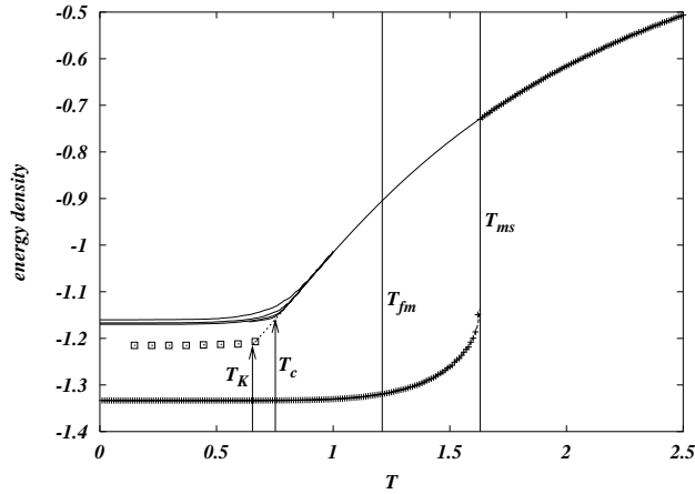
FIG. 1. Average energy as a function of the temperature for the ferromagnetic triangular plaquette model, on a Bethe hyperlattice where each spin belongs to k = 4 plaquettes (from[22]). If one prepares the system at low temperature in its ferromagnetic configuration s_i = 1 , and heats it up, the energy follows the bottom curve. At temperature T_{fm} the ferromagnetic state becomes metastable, but the system stays in this metastable ferromagnetic state until the spinodal temperature T_{ms} is reached. It then becomes paramagnetic. Cooling down from the paramagnetic state, the energy follows the upper curve, where the magnetization is zero. Below T_{fm} one is in a regime of supercooled paramagnetic state. In the temperature range below .9, one sees the effects of the cooling rate dependance on the energy (cooling rates from 10^2 to 10^5 MCS per \Delta T = 0.01 ). The theory predicts that at infinitely slow cooling there is a dynamical transition at T_c , where the energy is blocked at a threshold value, while the equilibrium ideal glass transition takes place at T_K , and the equilibrium energy density below T_K is given by the squares. It is conjectured that in finite dimensional models the temperature T_c marks the onset of activated processes: the energy can decrease slowly, and the real transition takes place at T_K .
