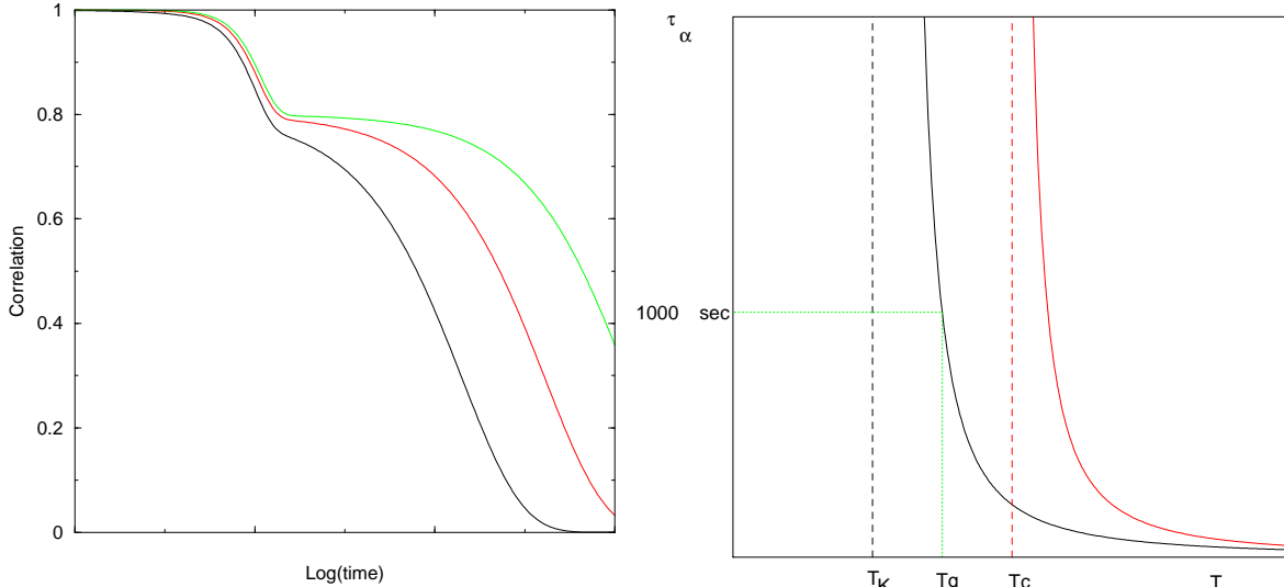
FIG. 2. The left-hand figure shows the schematic behaviour of the correlation function found in mean field discontinuous spin glasses and observed in structural glasses. The typical two-step relaxation consists of a fast \beta relaxation leading to a plateau, followed by a \alpha relaxation from the plateau, whose typical time scale increases rapidly when T decreases, and diverges at T = T_c which is equal to the mode-coupling transition temperature. The right-hand figure shows the behaviour of the relaxation time versus temperature. The right-hand curve is the prediction of mode-coupling theory without any activated processes: it is a mean field prediction, which is exact for instance in the discontinuous mean-field spin glasses. The left-hand curve is the observed relaxation time in a glass. The mode coupling theory provides a quantitative prediction for the increase of the relaxation time when decreasing temperature, at high enough temperature (well above the mode coupling transition T_c ) [24,25]. The departure from the mean field prediction at lower temperatures is usually attributed to 'hopping' or 'activated' processes, in which the system is trapped for a long time in some valleys, but can eventually jump out of it. The ideal glass transition, which takes place at T_K , cannot be observed directly since the system becomes out of equilibrium on laboratory time scales at the 'glass temperature' T_g .
