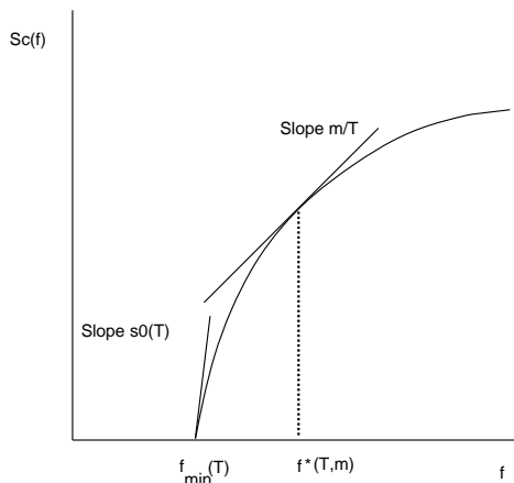
FIG. 3. Qualitative shape of the complexity versus free energy in mean field discontinuous spin glasses. The whole curve depends on the temperature. The saddle point which dominates the partition function, for m constrained replicas, is the point f^* such that the slope of the curve equals m/T (for the usual unreplicated system, m = 1 ). If the temperature is small enough the saddle point sticks to the minimum f = f_{min} and the system is in its glass phase. For m = 1 , this equilibrium phase transition happens at T = T_K .
