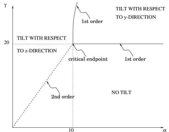
FIG. 10: Phase diagram of the elastic wall: \gamma_D as a function of \alpha_{\perp} .
