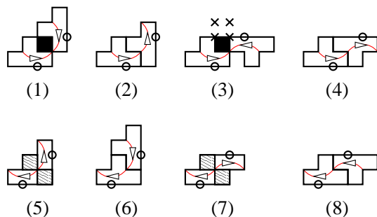
Figure 5: Arrow conservation at tile junctions.
