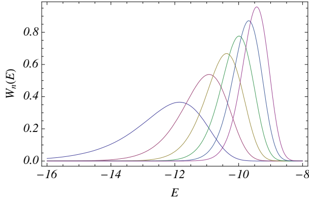
Figure 3: n th energy-level distribution W_n(E) for 1 \leq n \leq 6 with g = 10 , \sigma = 1 and L = 10^4 . We see from eqs. (61,62) that the dependence in n of the typical energy level and the width are E_n^{\text{typ}} \simeq E_1^{\text{typ}} + \frac{1}{\pi}\sqrt{g\sigma}\ln(n) and \delta E_n \simeq \delta E_1/\sqrt{n} , respectively.
