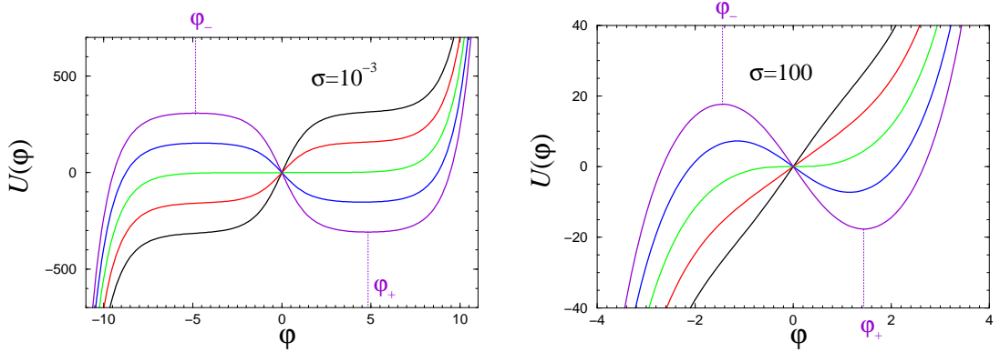
Figure 1: Potential U(\varphi) for g = 1 . Left : \sigma = 0.001 with energy E = 10, 5, 0, -5, -10 . Right : \sigma = 100 with energy E = 100, 50, 0, -50, -100 .
