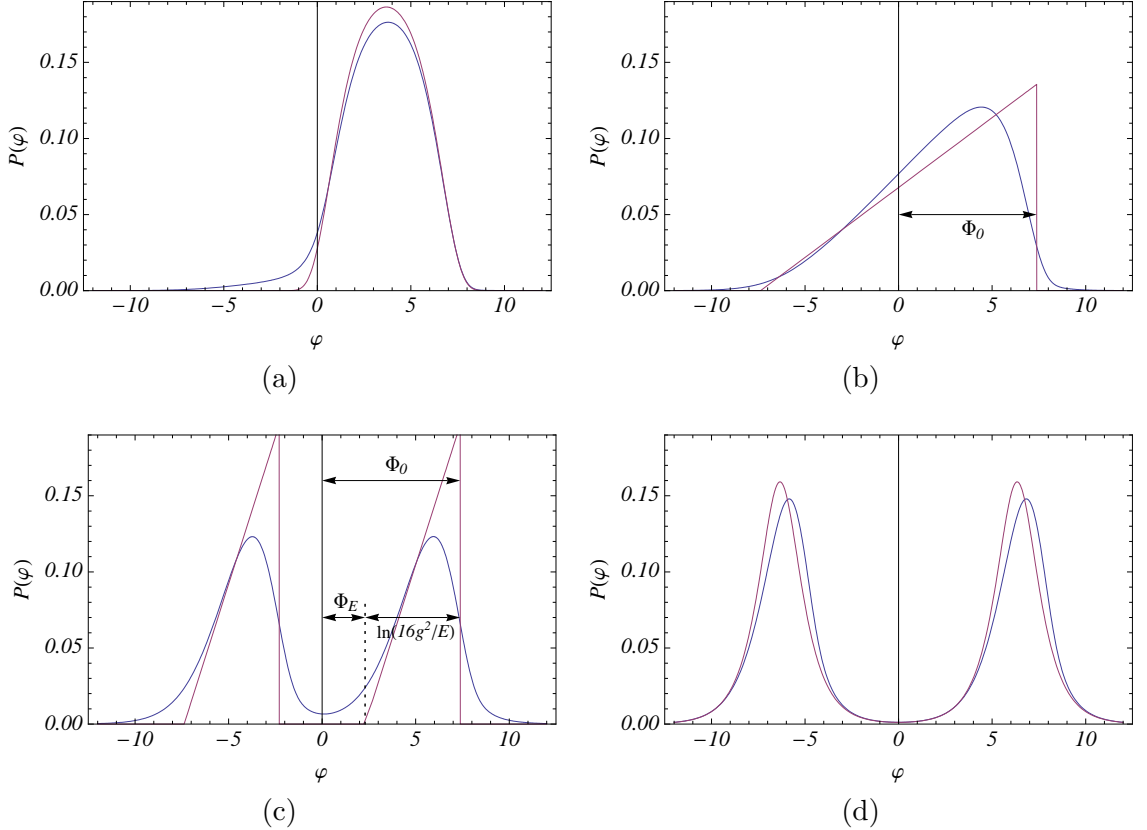
Figure 2: Distribution \mathcal{P}(\varphi) (blue curves) for (a) E = -0.01 , (b) E = 0 , (c) E = 0.1 and (d) E = 2 (with \sigma = 10^{-4} & g = 1 ). These behaviours can be understood from the shapes of the potential of the left part of figure 1. For E = -\sqrt{\sigma g} = -0.01 : the distribution is compared to \exp[-\frac{1}{g}\sqrt{|E|} \cosh(\varphi - \varphi_+)] . For the other energies, the distribution is compared to approximations obtained in the text.
