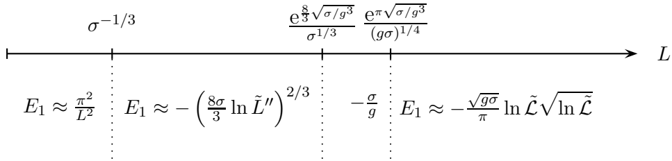
Figure 5: Illustration of regimes for the typical groundstate energy E_1 with increasing system sizes L in the small supersymmetric noise limit g^3 \ll \sigma . We recall that \tilde{\mathcal{L}} = \tilde{L}e^{-\frac{\pi}{4}\sqrt{\sigma/g^3}} .
